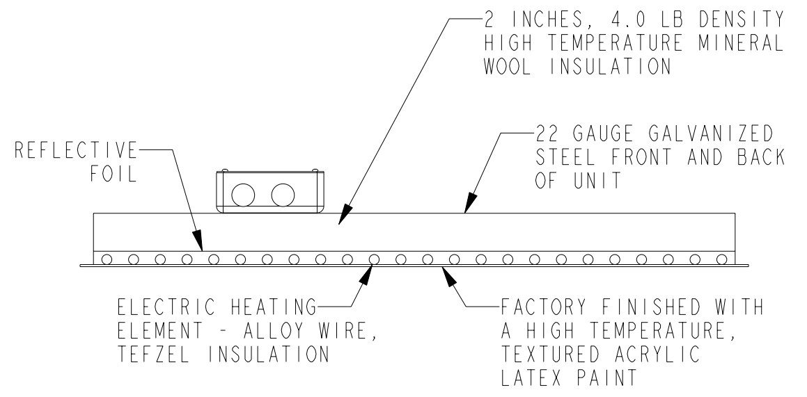
CUTAWAY VIEW OF SMARTROOMS ARCHITECTURAL SERIES HEATER
